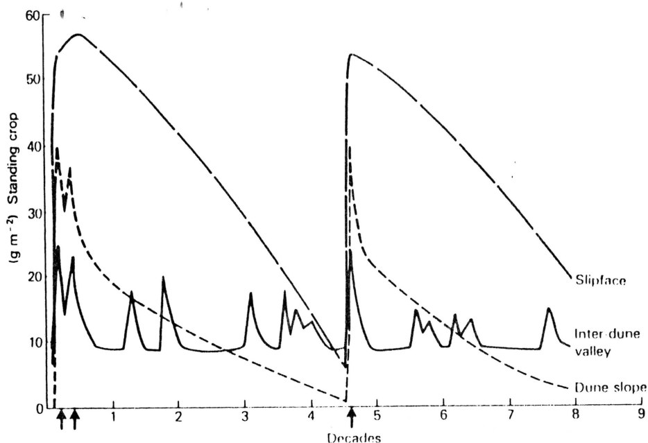
Fig. 2. - This simple model, based upon measurements of high and low biomass values measured in the Namib Desert of western Namibia (Louw & Seely, 1982), indicates the types of inter-annual variation of biomass that can be expected in an arid area. Similar variations would be expected in semi-arid or sub-humid areas, although the absolute values would differ from those portrayed. Such natural variation represents the major challenge for people attempting to make a living from drylands as well as for governments in dryland areas.
